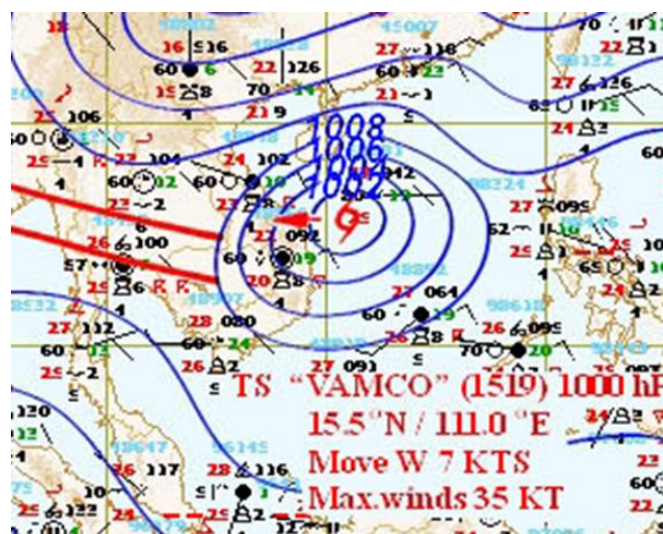
Figure 2: Weather map for 13 th September 2015
