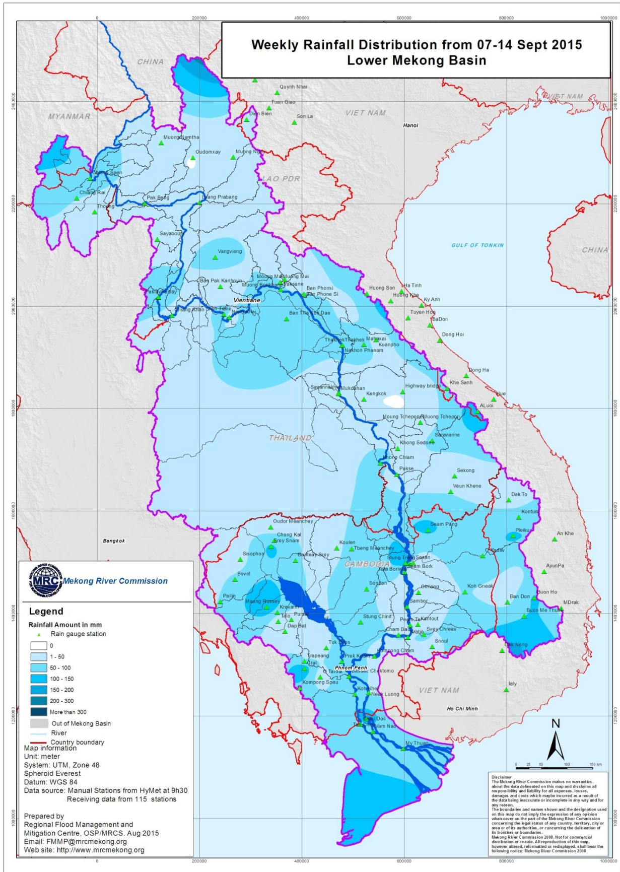
Figure 3: Weekly Rainfall Distribution over the LMB from 07 th – 14 th September 2015
